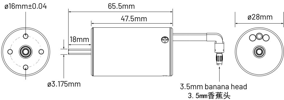
Appearance diagram 外观示意图 (±0.1-0.5mm)
